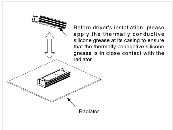
Schematic Diagram
