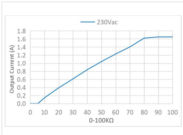
Rx Dimming Curve of Dim-to-off Version (linear)
