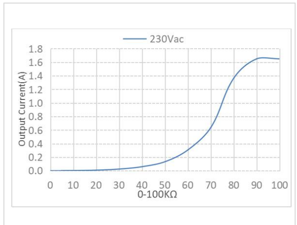
Rx Dimming Curve of Dim-to-off Version (logarithmic)
