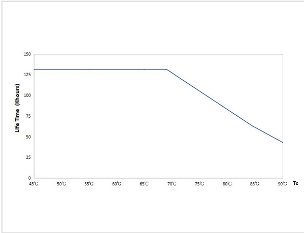
Lifetime Curve
