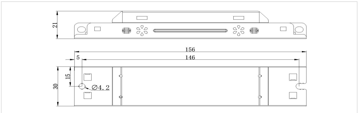
Structure Diagram
