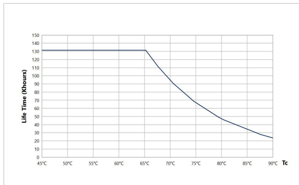
Lifetime Curve
