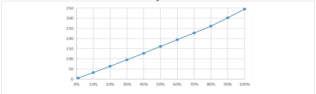
Dimming Curve
