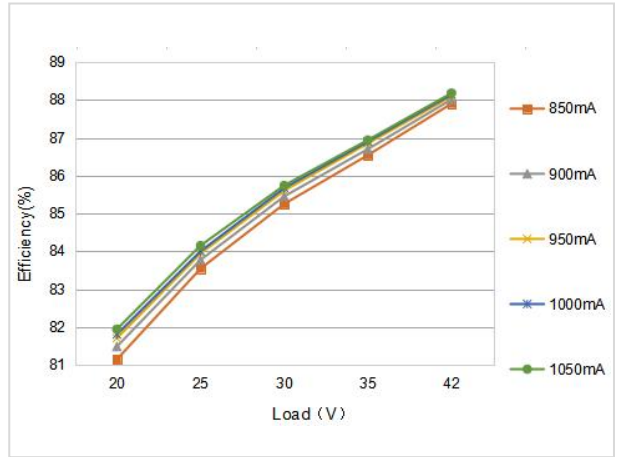
Efficiency Curve 2
