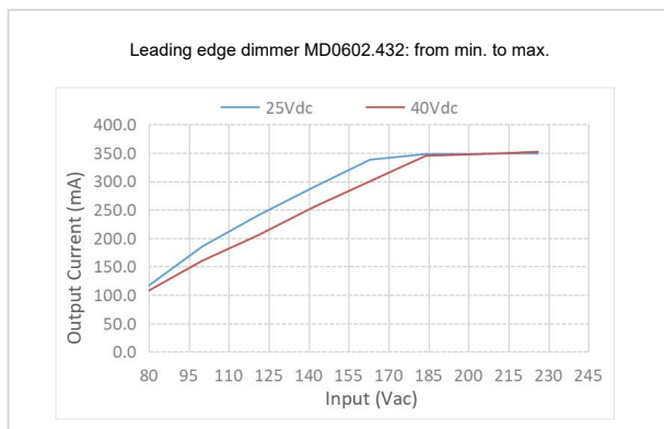
Leading Edge Dimmer MD0602.432: Minimum to Maximum Dimming Curve
