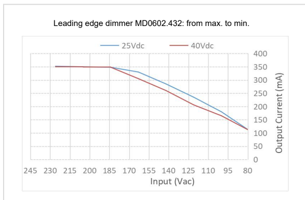
Leading Edge Dimmer MD0602.432: Maximum to Minimum Dimming Curve
